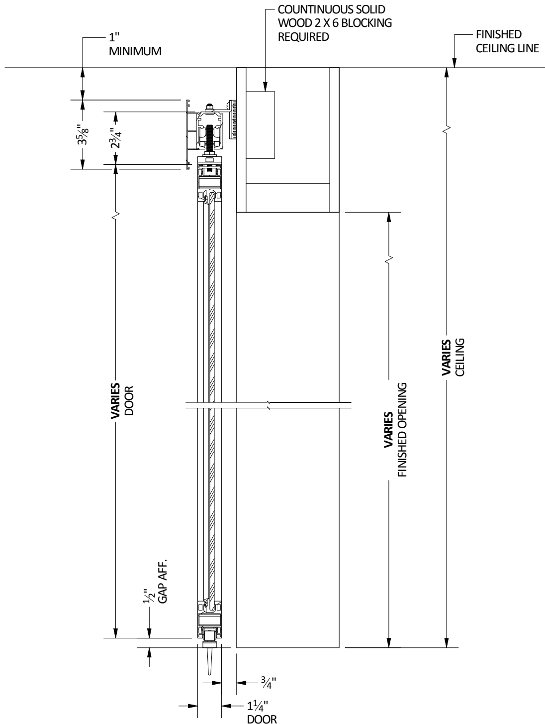
BDH6220EXX SYSTEM WITH METAL DOOR
